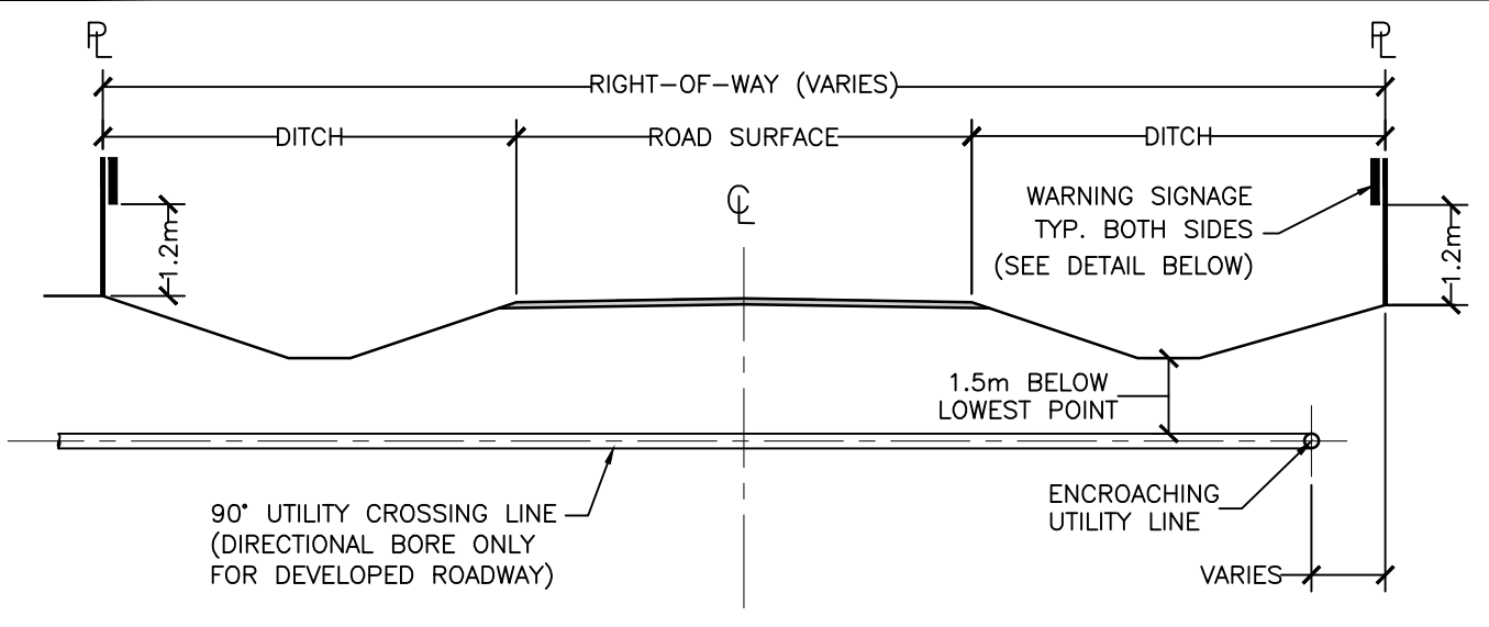
SECTION VIEW
